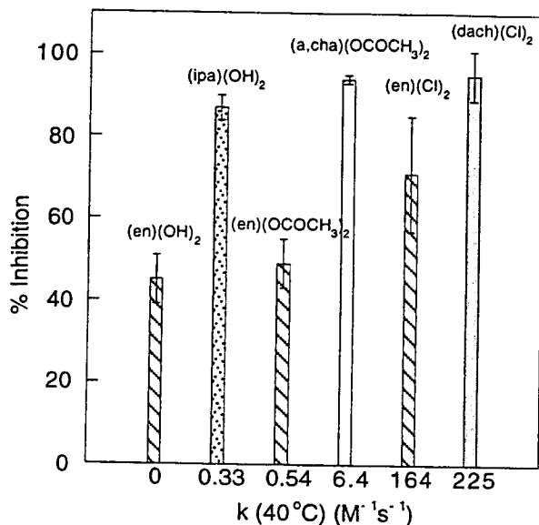
Figure 5. Percent growth inhibition of L1210/0 cells by Pt IV complexes versus reduction rate constant ( k , 40 °C) of Pt IV complexes by ascorbic acid; % inhibition = 100[1 - (N_D/N_{D0})/(N_C/N_{C0})] , where N_D , N_{D0} , N_C , and N_{C0} are the number of cells ( \sim 10^5 – 10^6 cells/mL) treated with a Pt IV compound (7 \mu M) and saline solution (0.1 M NaCl) at time t (3 days) and 0, respectively. Each value represents the mean \pm the standard error of at least two independent experiments.
