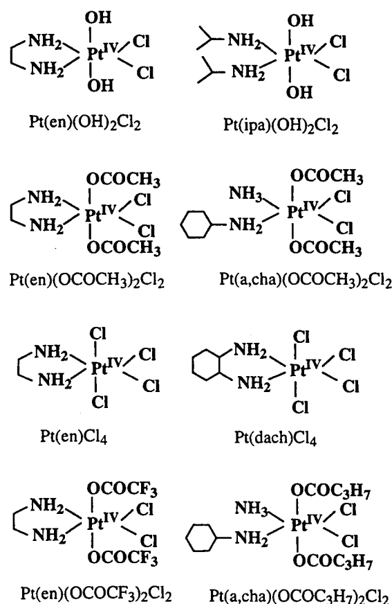
Figure 1. Molecular structures of Pt IV complexes studied in this research.
