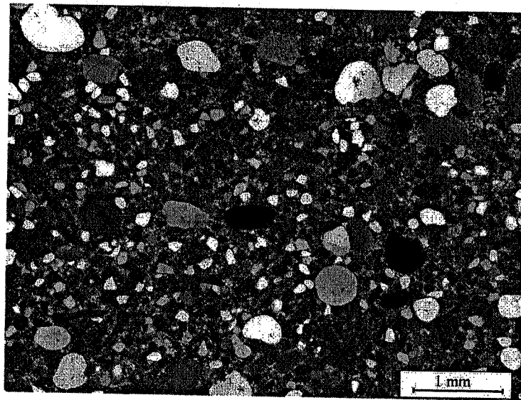
Figure 4. Bimodal distribution of quartz sediment in Ticonderoga Formation, with rounded sand grains and angular silt grains. Note subparallel arrangement of sand and silt layers (angled approximately 30° counterclockwise from horizontal in this particular view). Crossed polars.
