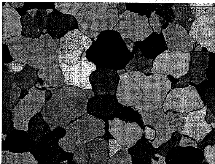
Figure 1. Photomicrograph of Potsdam Formation. Crossed polars. The quartz sand grains are well rounded, and show numerous fluid inclusions. In most cases, the quartz cement is optically continuous.
