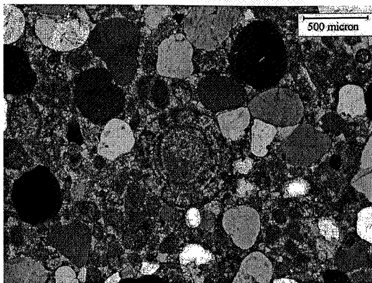
Figure 2. Photomicrograph of Ticonderoga Formation. Crossed polars. Note large, rounded quartz grains, peloids (small, rounded, dark masses), and oolite in center, showing characteristic radial structure around its core.
