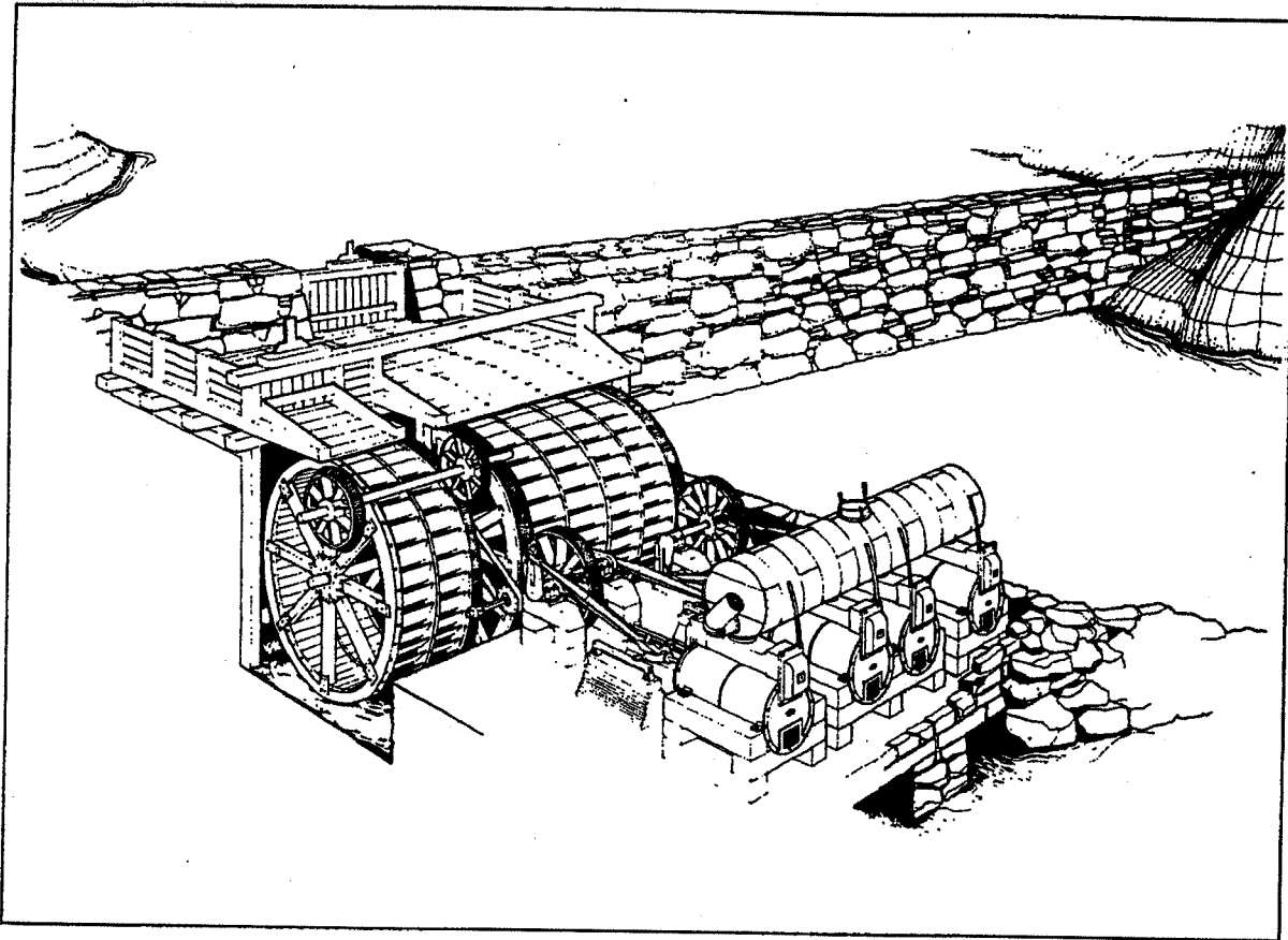
Figure 4. Reconstruction of the dam and blowing engine of the "new" furnace.
